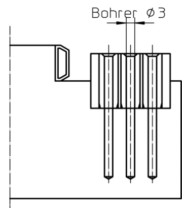
cross section
