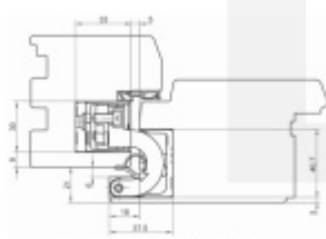
Example overlap thickness 21 mm
